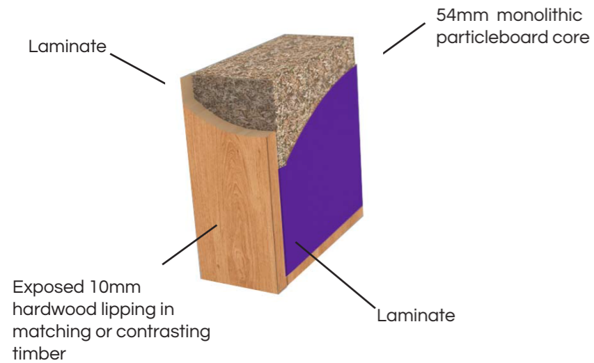
Standard detail of heavy duty core
