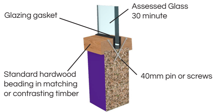
Standard detail of vision panel glazing
